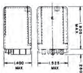
PR-26 Dimensions
